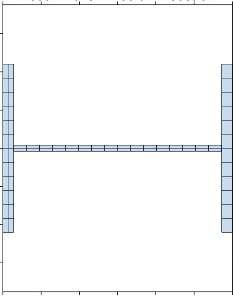
H300x220x8x14 column section
